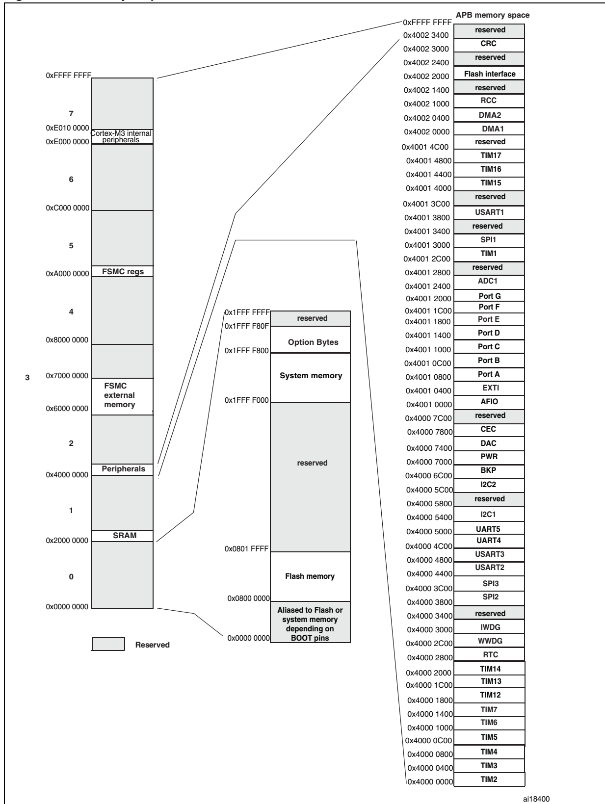
Figure 6. Memory map
