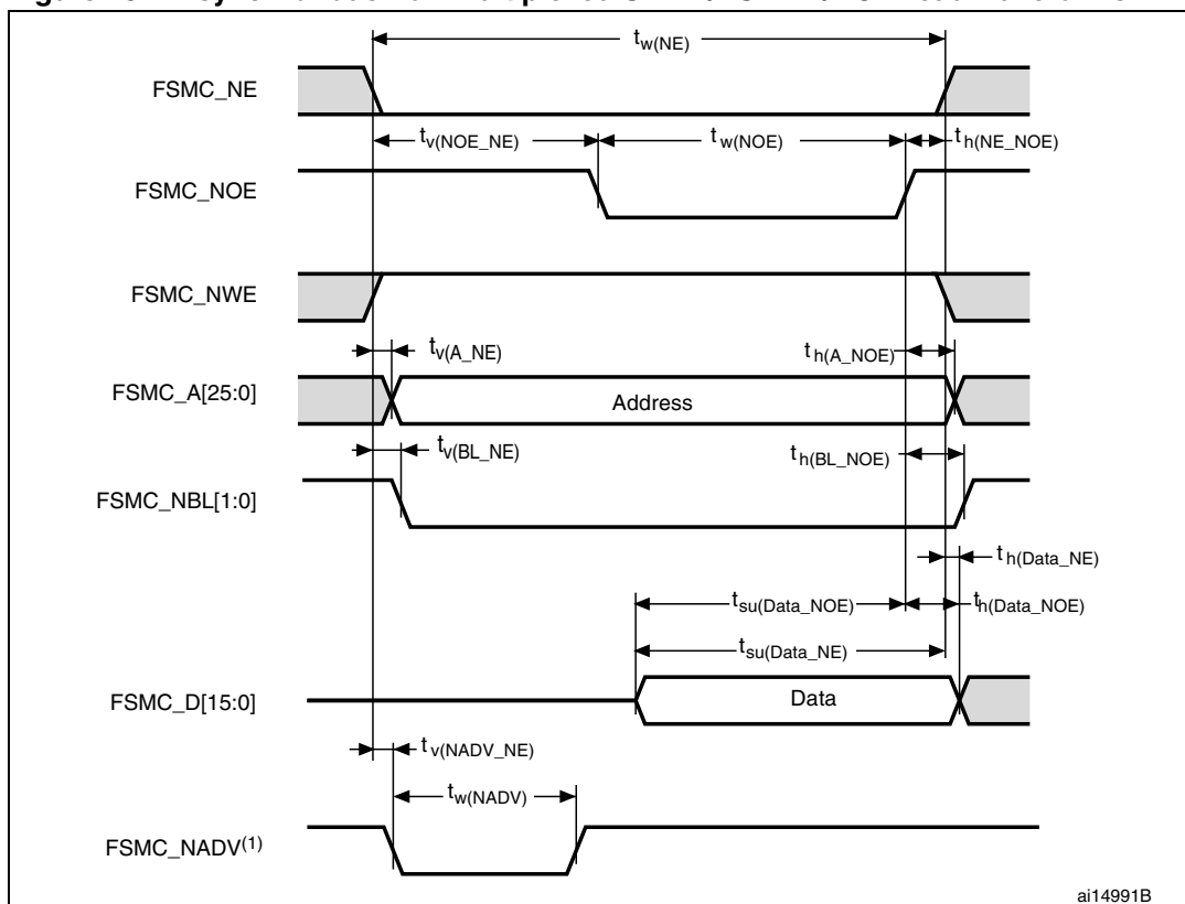
Figure 15. Asynchronous non-multiplexed SRAM/PSRAM/NOR read waveforms
