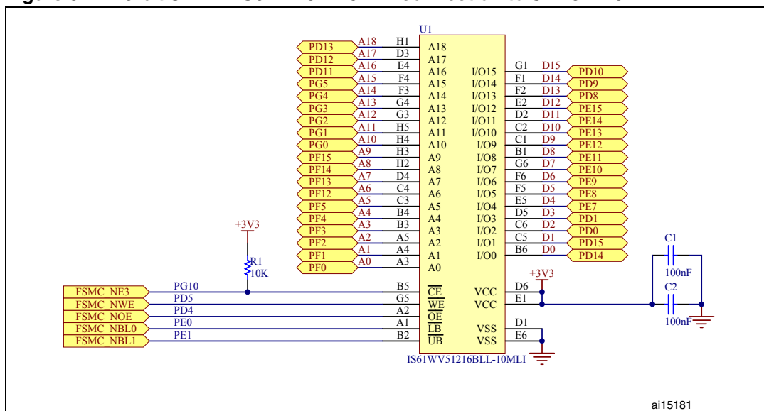
Figure 8. 16-bit SRAM: IS61WV51216BLL connection to STM32F10xxx
