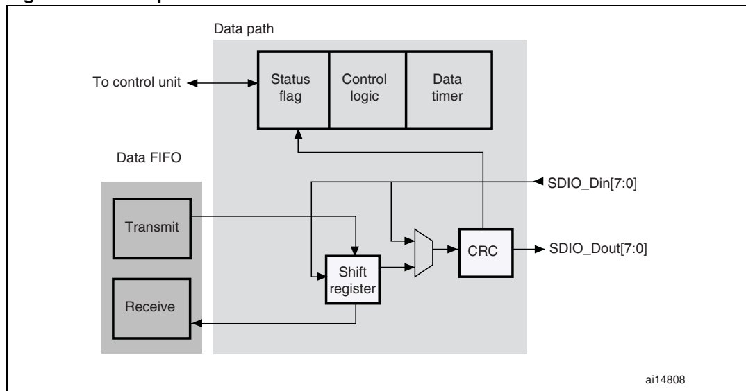
Figure 217. Data path
