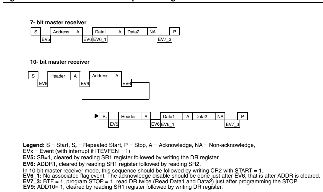
Figure 275. Method 2: transfer sequence diagram for master receiver when N=2
