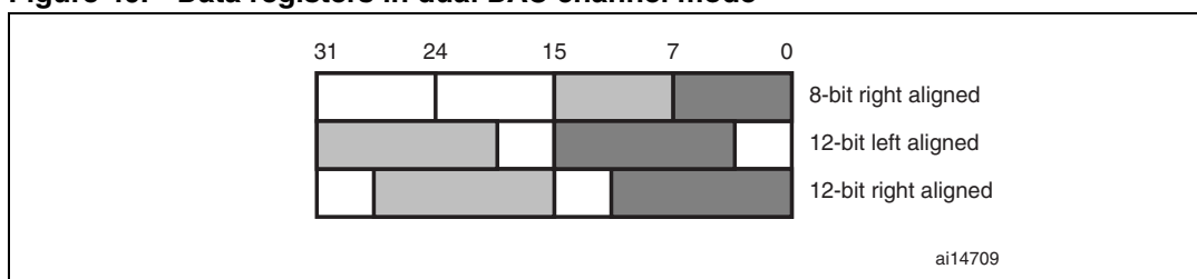
Figure 46. Data registers in dual DAC channel mode
